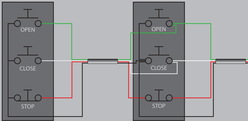
Double 3-Button Stations
