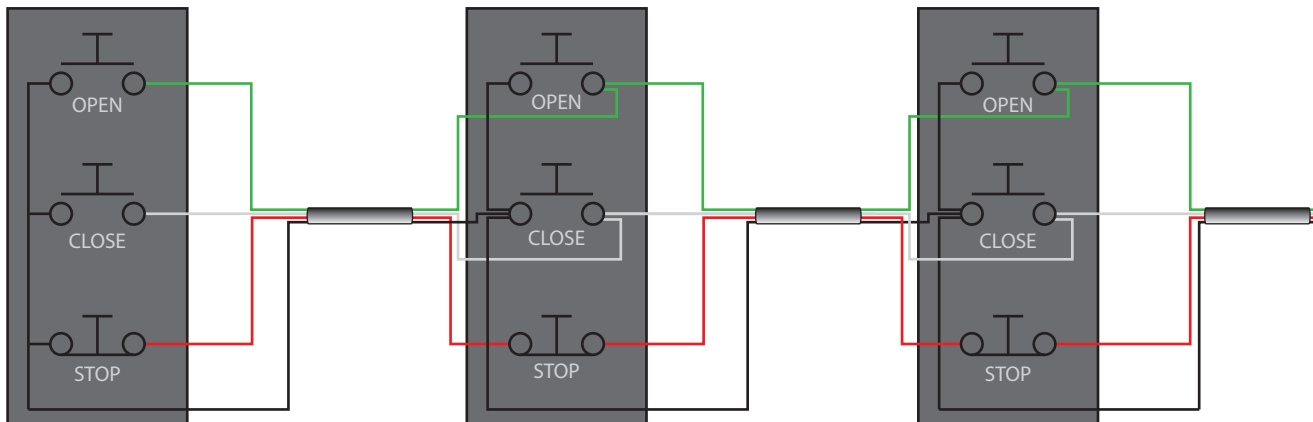
Multiple 3-Button Stations Refer to the operator manual to verify wiring connections
