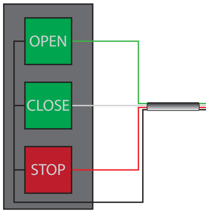
Single 3-Button Station
