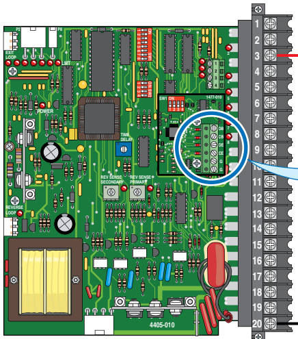
6-Pin UL 325 Terminal Entrapment Protection Device Connection
