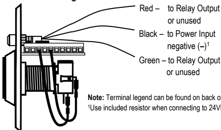
Figure 9 - Side View
